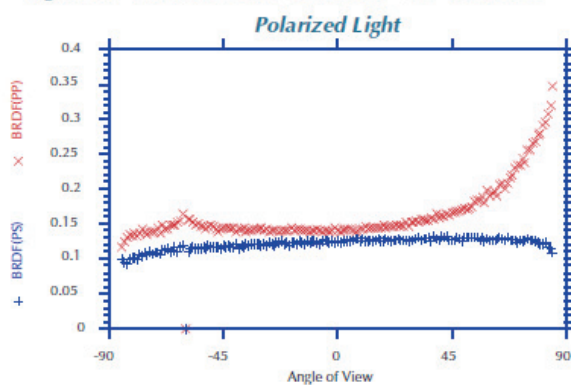
Figure 17 - In-Plane BRDF at 633 nm - 60° Incidence
