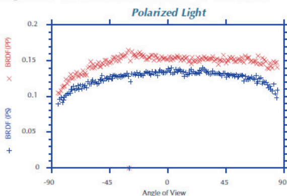
Figure 16 - In-Plane BRDF at 633 nm - 30° Incidence
